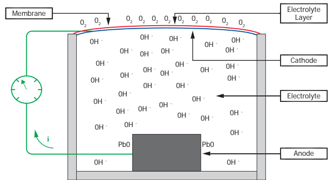
Sensor Construction
